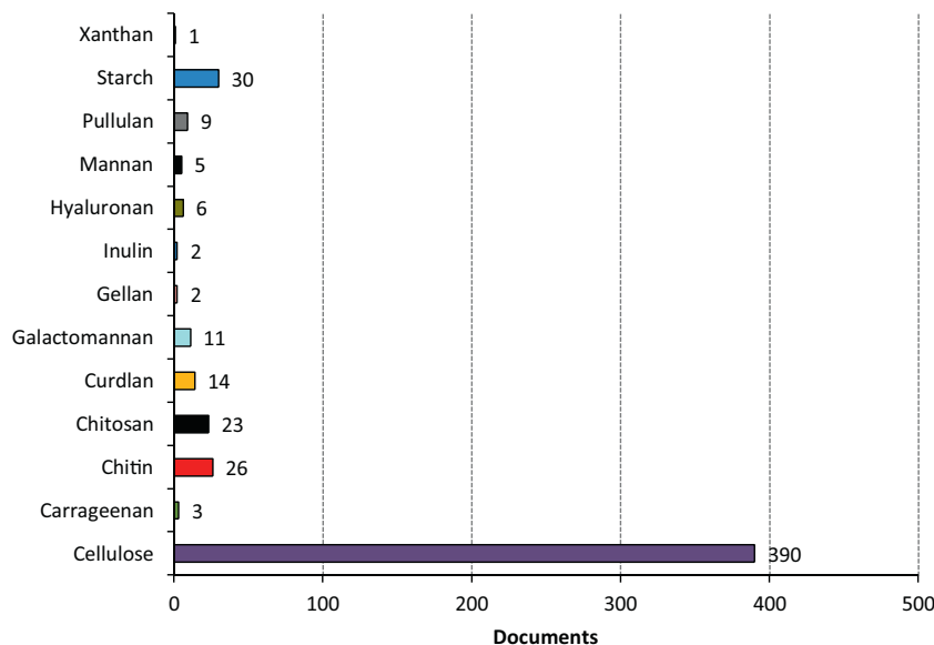
Fig. 3. Document search results since 2000 on Scopus website using specific keywords association "TEMPO" and "oxidation" and a variable one.
