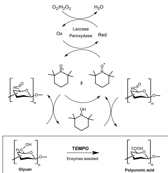
Fig. 5. Mechanisms of glycan oxidation by TEMPO/laccase/O 2 or TEMPO/perydoxase/H 2 O 2 systems, adapted from Bragd et al. (2004).
