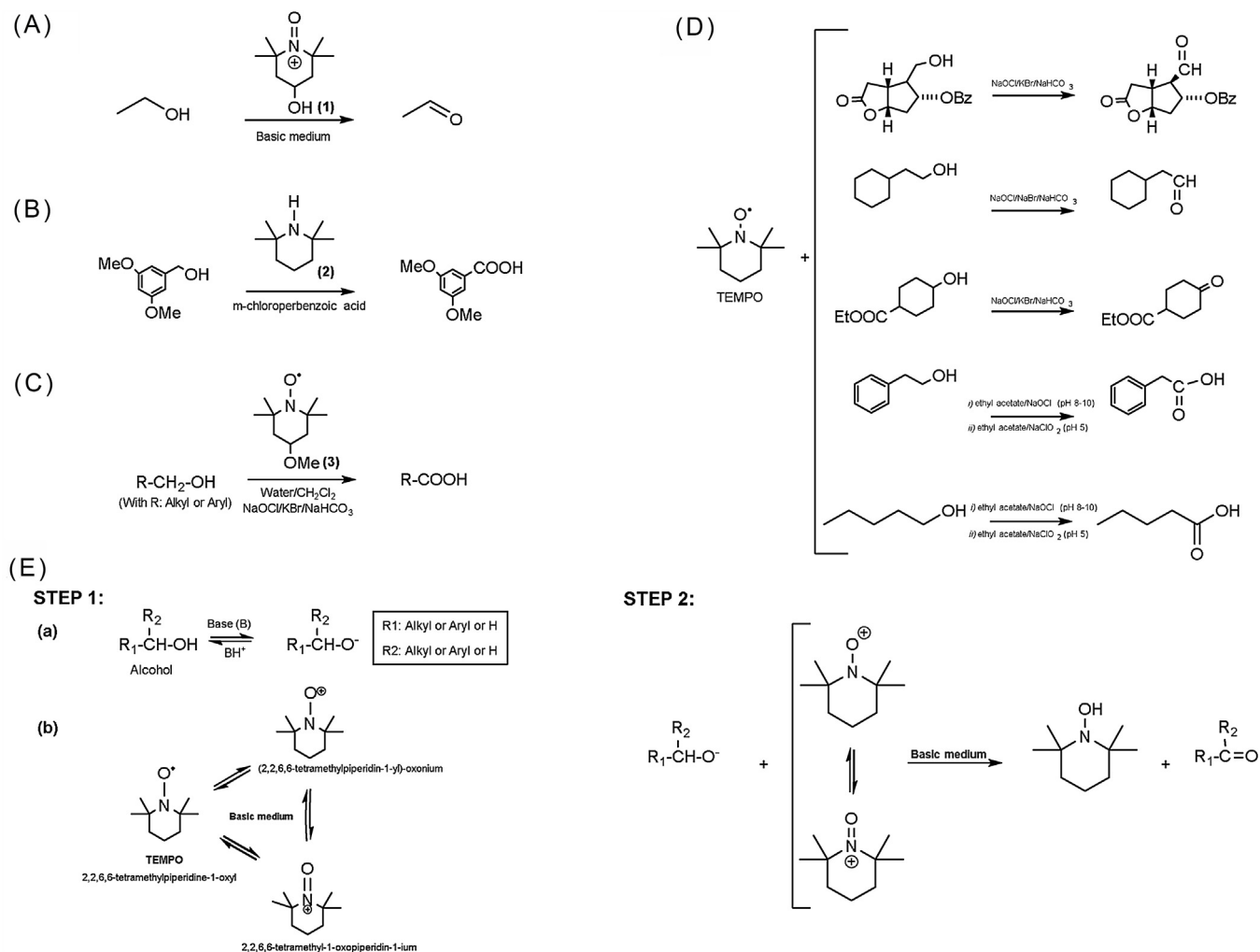
Fig. 2. Examples of alcoholic compounds oxidation strategies using TEMPO and derivatives. (A) Oxidation of ethanol onto acetaldehyde using 4-hydroxy-2,2,6,6-tetramethyl-1-oxopiperidin-1-ium (1) (adapted from Golubev et al., 1966); (B) oxidation of (3,5-dimethoxyphenyl)-methanol onto 3,5-dimethoxybenzoic acid using 2,2,6,6-tetramethylpiperidine (2) and m -chloroperbenzoic acid (adapted from Cella et al., 1975); (C) general oxidation of alcohol onto carboxylic acid using Water/CH 2 Cl 2 biphasic system and 4-methoxy-TEMPO/NaOCl/KBr/NaHCO 3 (3) (adapted from Anelli et al., 1987); (D) examples of syntheses of ketones, aldehydes and carboxylic acid compounds by using TEMPO (adapted from Caron et al., 2006; Ciriminna & Pagliaro, 2010) and, (E) Alcohol oxidation mechanism under alkaline media using TEMPO (adapted from Bailey et al., 2007; Semmelhack, Schmid, & Cortes, 1986).
