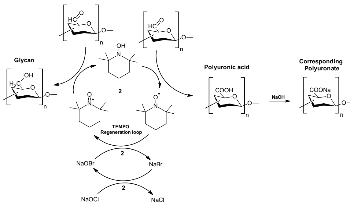
Fig. 4. TEMPO-mediated oxidation of glycans to generate their corresponding polyuronates with NaOCl/NaBr system, adapted from Elboutachfai, Delattre et al. (2011).
