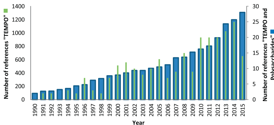
Fig. 1. Number of references per year between 1990 and 2015 using the key words "TEMPO" and the combination "TEMPO and Polysaccharides".
