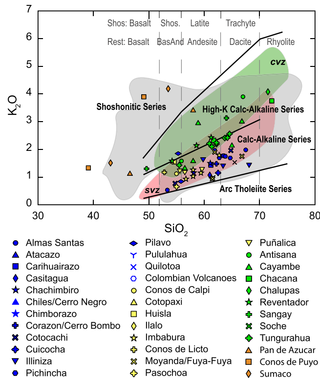
Figure 3. SiO 2 versus K 2 O diagram of Peccerillo and Taylor [1976] classifying arc rock types. Samples from the literature are represented by the gray-shaded area [Barragan et al., 1998; Bourdon et al., 2002a, 2002b; Bourdon et al., 2003; Samaniego et al., 2005; Bryant et al., 2006; Hidalgo et al., 2007; Robin et al., 2008; Hoffer et al., 2008; Chiaradia et al., 2009; Schiano et al., 2010; Samaniego et al., 2010; Samaniego et al., 2011; Chiaradia et al., 2011; Garrison et al., 2011; Hidalgo et al., 2012] and samples from this study are displayed (see supporting information). Volcano geological setting is color coded according to: blue = Western Cordillera (WC), Yellow = Inter-Andean Valley (IV), Green = Eastern Cordillera (EC), Orange = Back-Arc (BA). Arc zonation is visible as alkaline content at given SiO 2 increases away from the trench. Composition of other Andean volcanic zones are displayed, the Central Volcanic Zone (CVZ) by the green shaded area [Davidson and de Silva, 1992; Feeley and Davidson, 1994; Delacour et al., 2007; Hora et al., 2007; Mamani et al., 2008, 2010; Sørensen and Holm, 2008] and the Southern Volcanic Zone (SVZ) by the red shaded area [Hickey-Vargas et al., 2016].
