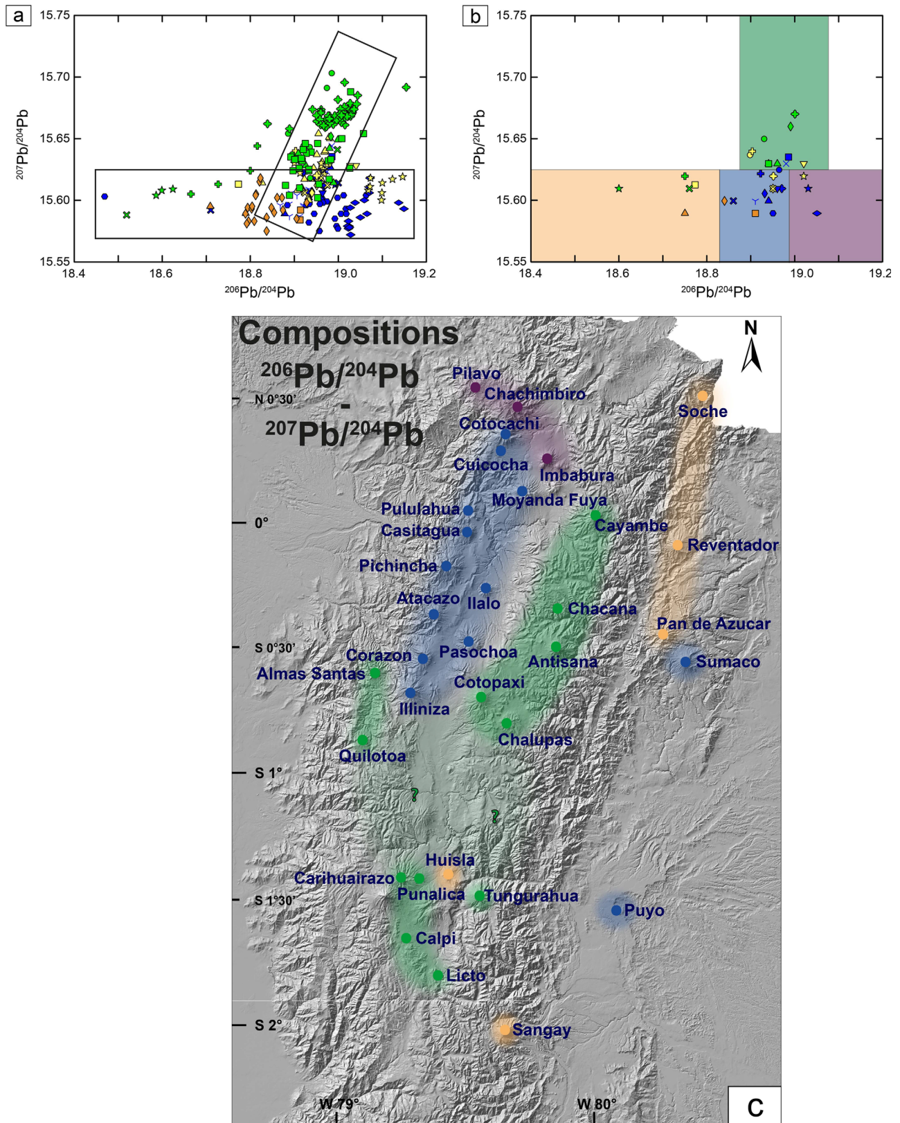
Figure 9. (a) ^{207}\text{Pb}/^{204}\text{Pb} versus ^{206}\text{Pb}/^{204}\text{Pb} diagram displaying Ecuadorian volcanic products (detail of Figure 6) and highlighting the trends discussed in the text. (b) ^{207}\text{Pb}/^{204}\text{Pb} versus ^{206}\text{Pb}/^{204}\text{Pb} diagram showing mean values for each volcano. Main isotopic signatures are color coded with blue representing the intersection of the two trends, and the other colors representing the extremities. (c) Geographical distribution of the main lead isotopic signatures; colors as in Figure 9b.
