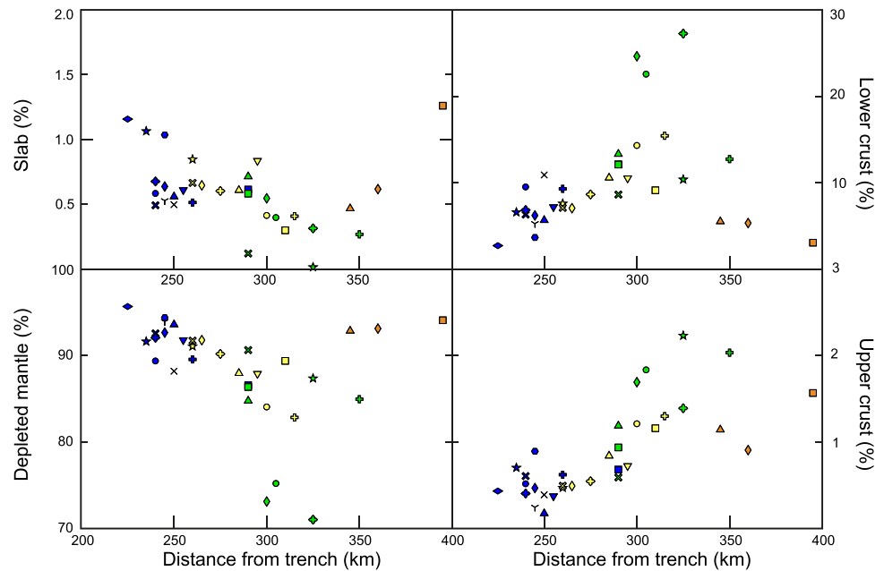
Figure 13. Mass-balance model. The mass fractions of upper crust, lower crust, mantle melts, and slab component at each volcanic center are plotted against distance from trench. Legend as in Figures 3 and 10.
