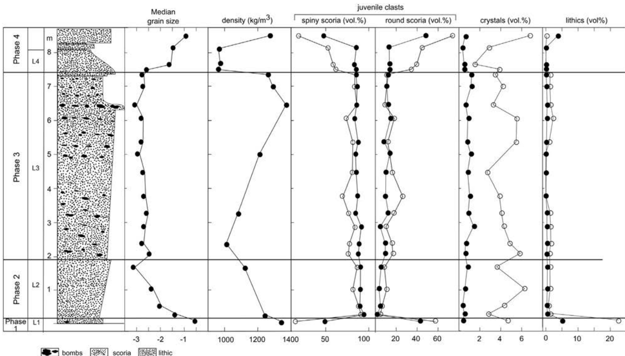
Fig. 10. Variations of median grain size, the main four clast components and the mean clast density within the proximal stratigraphic succession of the La Vache and Lassolas tephra deposit.
