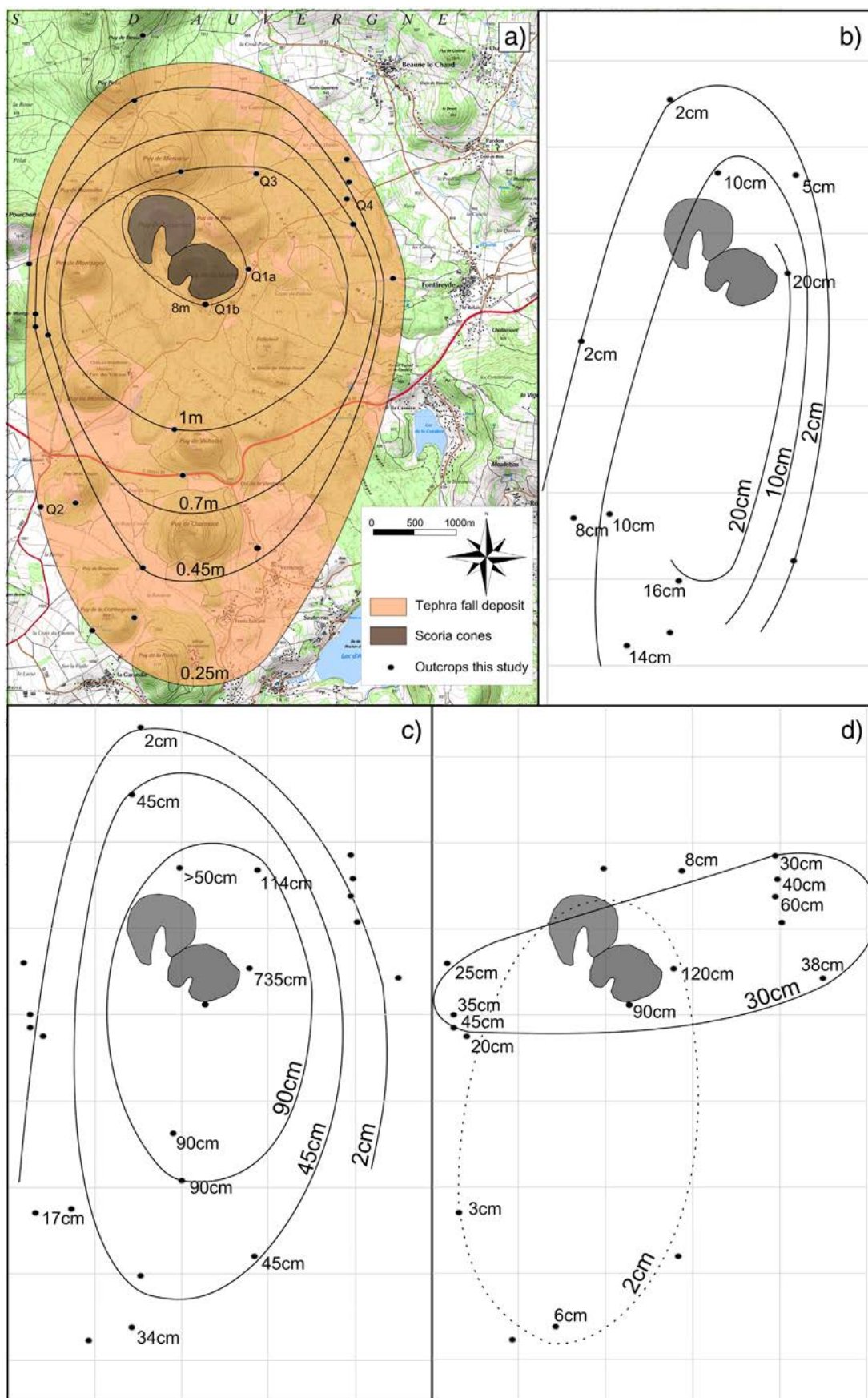
Fig. 8. Isopach maps for a) the total tephra deposit, b) the opening phase layer PL1, c) the second and third phase of the eruption (layer PL2 and PL3) and d) the main layer of the fourth phase (layer PL4).
