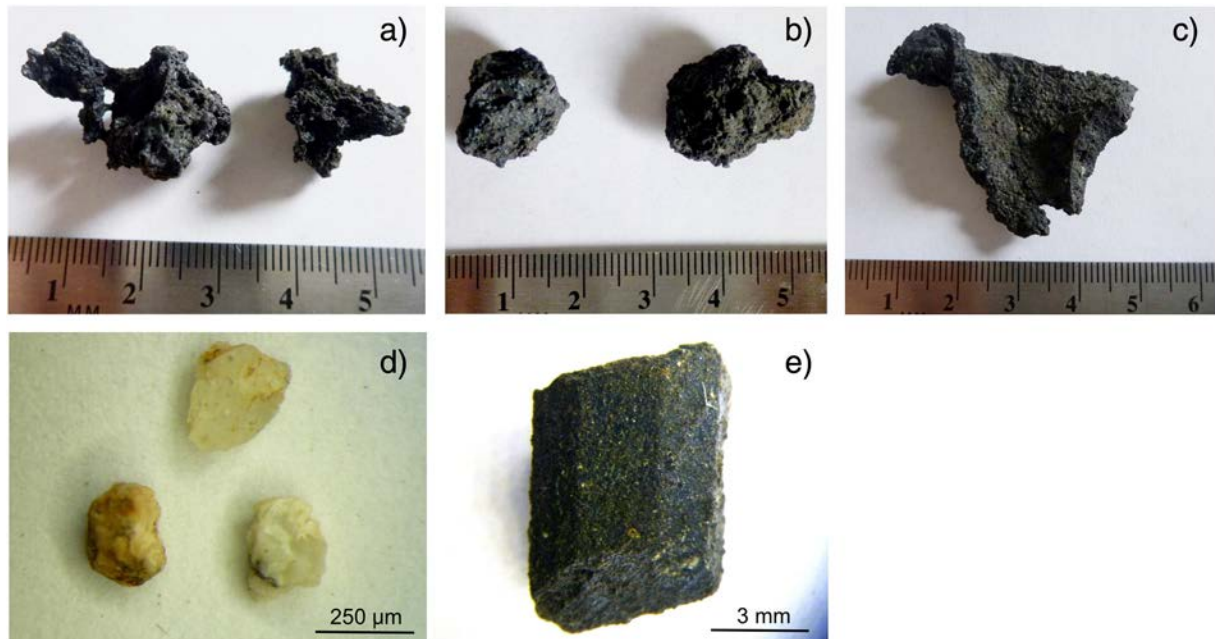
Fig. 3. Images of the five different clast types such as a) vesicular juvenile clasts, b) subrounded juvenile clasts, c) platy juvenile clasts, d) magmatic crystals and e) granitic lithic clasts.
