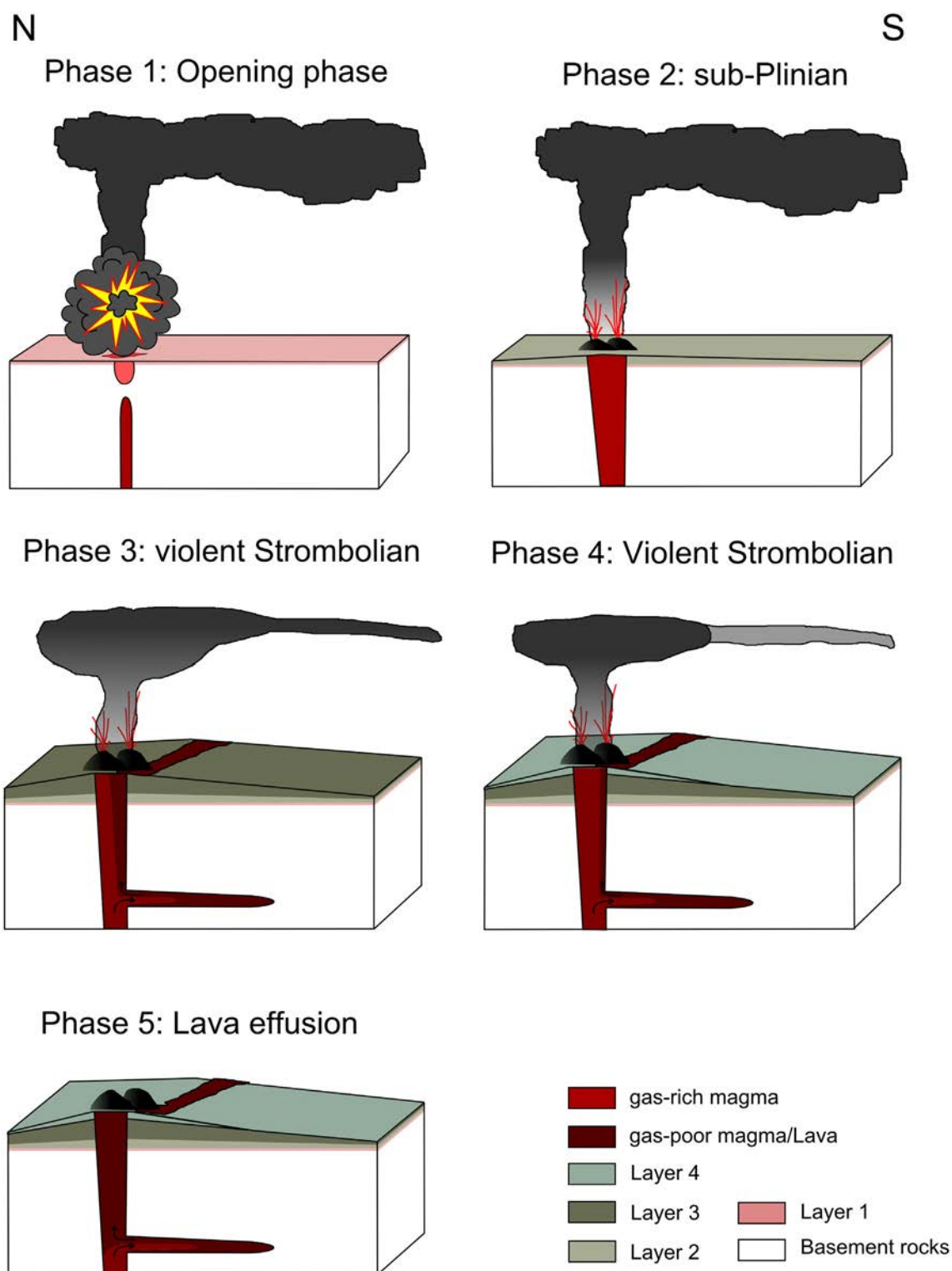
Fig. 11. Evolution of the eruption from a gas-driven explosive first vent opening phase, to a highly explosive cone-forming second phase, to less explosive violent Strombolian third and fourth phase and quiet lava effusion in the last phase of the eruption.
