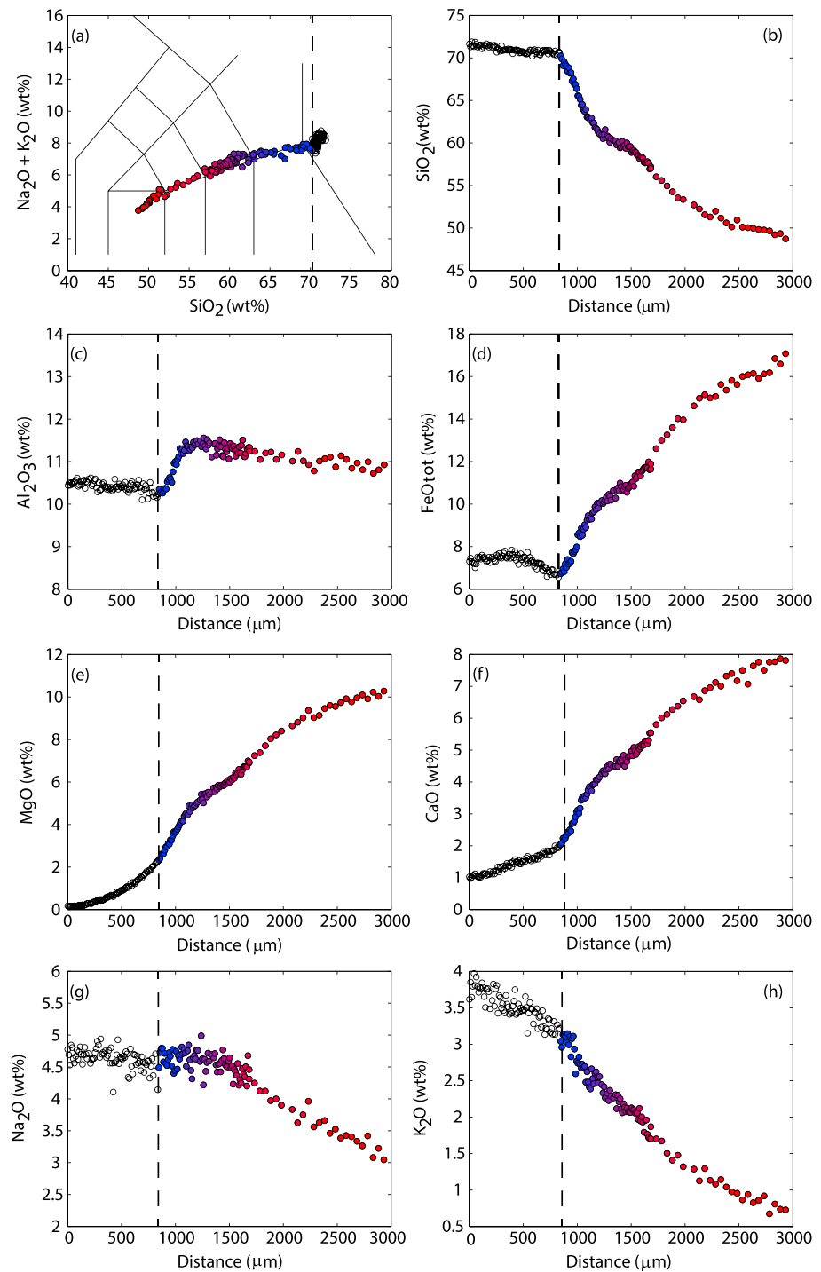
Figure 1. (a) TAS (total alkali versus SiO 2 contents in wt %) diagram showing the chemical composition of glasses used in this study; (b–h) measured chemical composition as a function of the distance along the analyzed glassy filament. The color scale (from red to blue) codifies the evolution of the chemical composition, along the investigated glassy filament. As the composition of the glass becomes more rhyolitic the symbol color becomes more blue. White symbols represent the chemical composition of glasses excluded to develop the model (see text).
