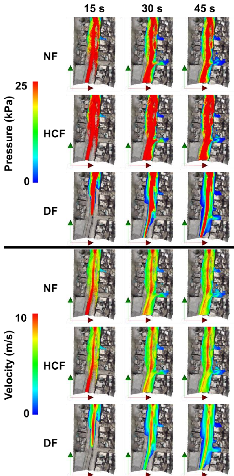
630 Figure 5. Evolution of dynamic pressure and velocity magnitudes for a 75 \text{ m}^3\text{s}^{-1} flow along Quebrada Dahlia for a Newtonian flow (NF), hyperconcentrated flow (HCF) and debris flow (DF). Arrows indicate North (green) and East (red) direction.
