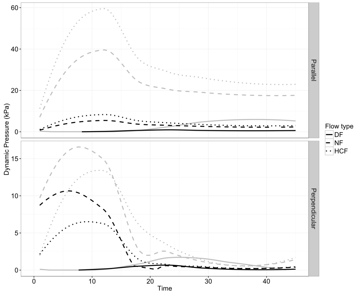
640 Figure 7. Comparison of mean pressure magnitude (grey lines) and mean normal pressure (black lines) on block ‘West 2’ in the parallel and perpendicular orientations for a 75 \text{ m}^3\text{s}^{-1} flow along Quebrada Dahlia.
