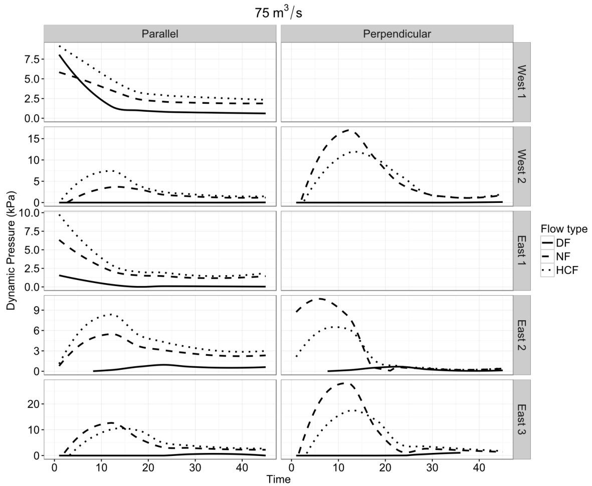
Figure 8. Mean normal pressures applied to each city block in the perpendicular and parallel orientations for a 75 \text{ m}^3/\text{s} flow.
