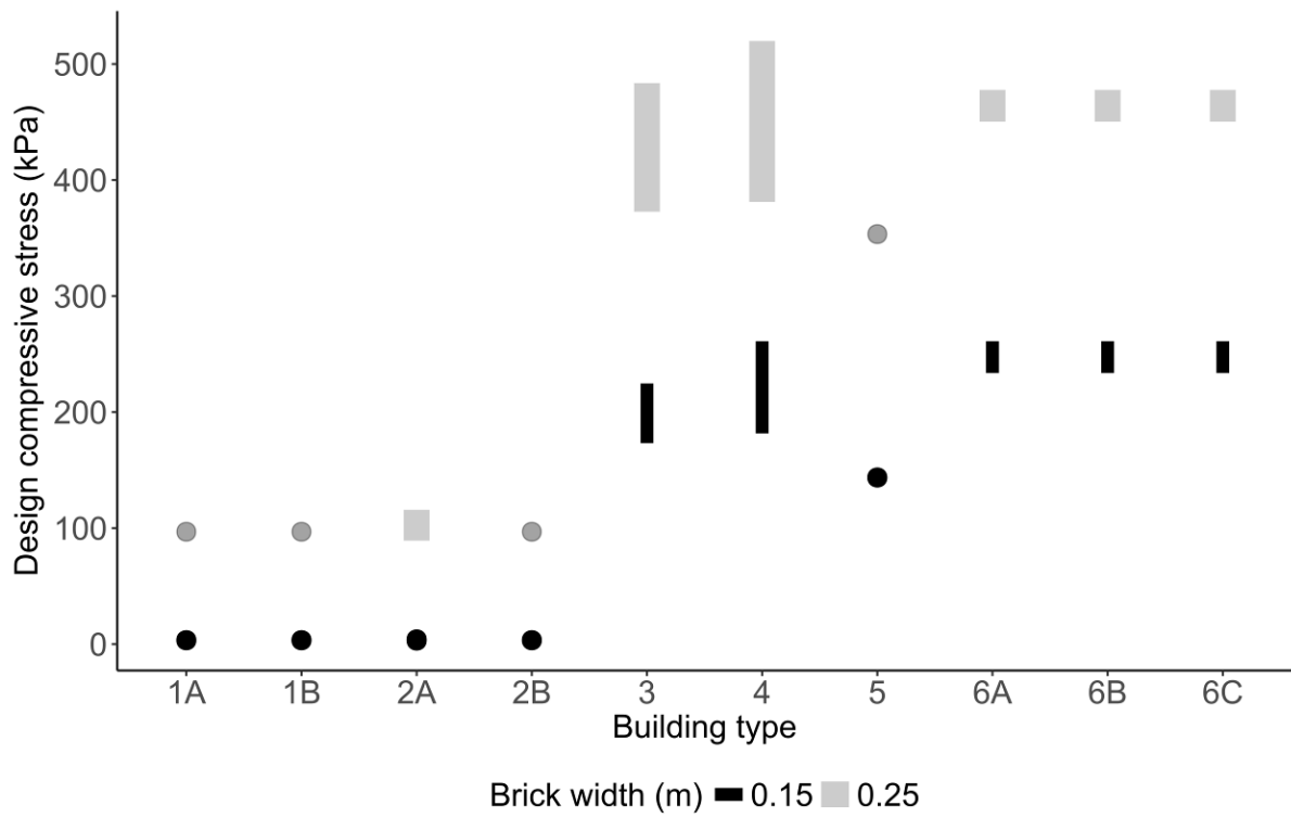
Figure 3. Range of design compressive stress for building types 1A - 6C defined in Thouret et al. (2014). Compressive stress capacity was calculated for every configuration of compressive strength ( f_c ), bedded area ( A_b ), and thickness coefficient ( k_t ) at brick widths ( b ) of 150 mm and 250 mm.
