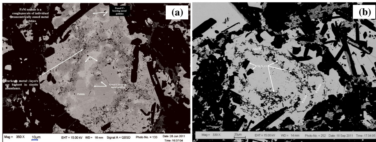
Fig. 4. a) A BSE-SEM photograph of metal nodule No. 17 in EL3 MS-17 fragment depicting the heterogeneous conglomerate of concentrically zoned metal pebbles. Cores of pebbles depict lower brightness due to higher C-content (arrows). These portions are also crowded with submicron crystallites of sinoite. b) A SEM-BSE photograph of nodule No. 34 in EL3 fragment MS-17. Nodule has a core encompassing numerous sinoite-decorated micropebbles with two large idiomorphic sinoite ( \text{Si}_2\text{N}_2\text{O} ) stubby crystals and is decorated by submicron crystallites of sinoite (white arrows). The core is covered by several metal pebbles and a metal shell. (Color figure can be viewed at wileyonlinelibrary.com .)
