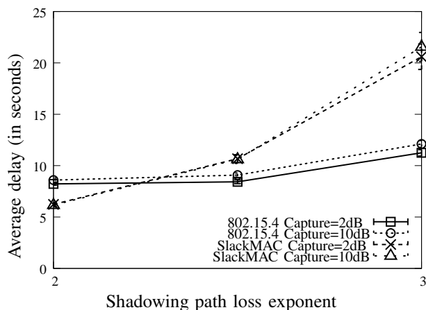
Fig. 6. Average delay as a function of the shadowing path loss exponent, with shadowing standard deviation of 4 dB for IEEE 802.15.4 and SlackMAC, when the capture threshold equal to 2 dB and 10 dB.
