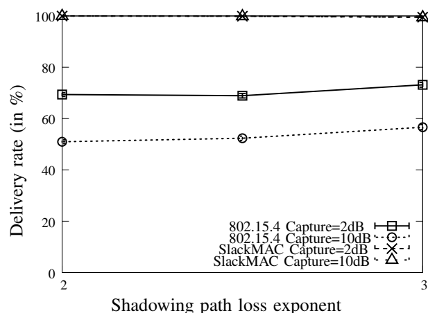
Fig. 5. Delivery rate as a function of the shadowing path loss exponent, with shadowing standard deviation of 4 dB for IEEE 802.15.4 and SlackMAC, when the capture threshold equal to 2 dB and 10 dB.
