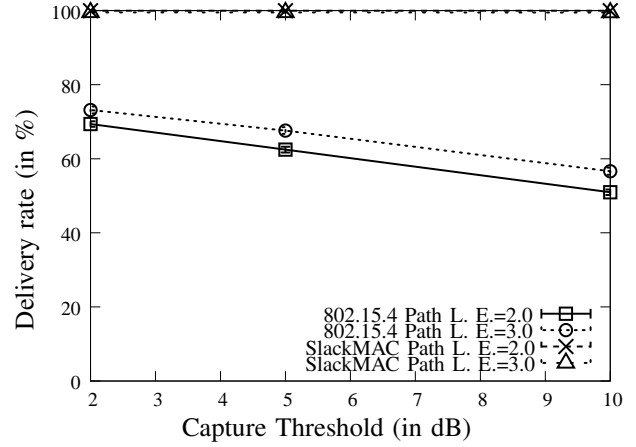
Fig. 3. Delivery rate as a function of the capture threshold with shadowing standard deviation of 4 dB for IEEE 802.15.4 and SlackMAC, when shadowing path loss exponent equal to 2.0 and 3.0.
