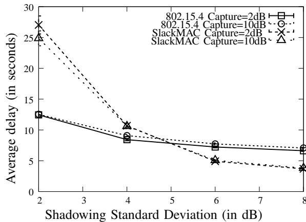
Fig. 8. Average delay as a function of the shadowing standard deviation, with shadowing path loss exponent of 2.5 for IEEE 802.15.4 and SlackMAC, when the capture threshold equal to 2 dB and 10 dB.
