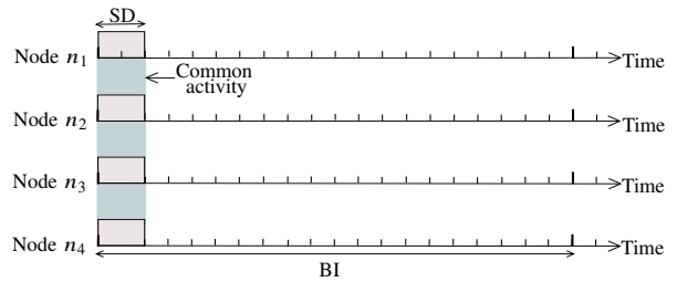
Fig. 1. Example of activity cycle of four nodes n_1, n_2, n_3 and n_4 in range, with a duty cycle of 10 % in the standard IEEE 802.15.4.
