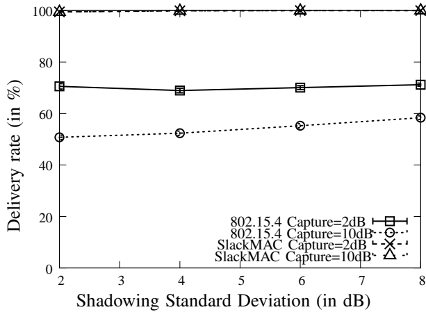
Fig. 7. Delivery rate as a function of the shadowing standard deviation, with shadowing path loss exponent of 2.5 for IEEE 802.15.4 and SlackMAC, when the capture threshold equal to 2 dB and 10 dB.
