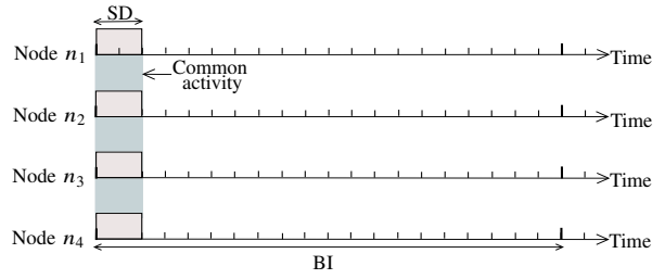
Fig. 1. Example of activity cycle of four nodes n_1, n_2, n_3 and n_4 in range, with a duty cycle of 10 % in the standard IEEE 802.15.4.
