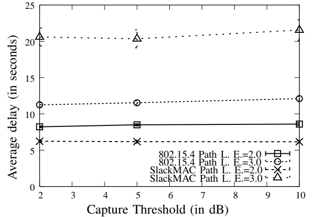
Fig. 4. Average delay as a function of the capture threshold with shadowing standard deviation of 4 dB for IEEE 802.15.4 and SlackMAC, when shadowing path loss exponent equal to 2.0 and 3.0.
