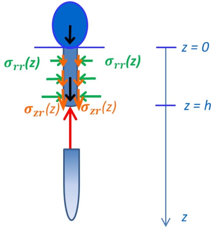
Fig.7: Schematic diagram of the forces resisting to the up-lifting of the root outside the soil due to growth in the constraining soil. The seedling is artificially decomposed into a growing part (bottom part) and a non-growing part (upper part) over which the balance of forces is made. The root axis z is aligned with gravity. The seed is just lying on the soil surface at z=0 and the non-growing part of the root is buried till the depth z=h .
