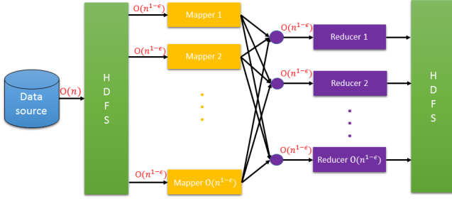
Figure 1: MapReduce flowchart with MRC constraints
