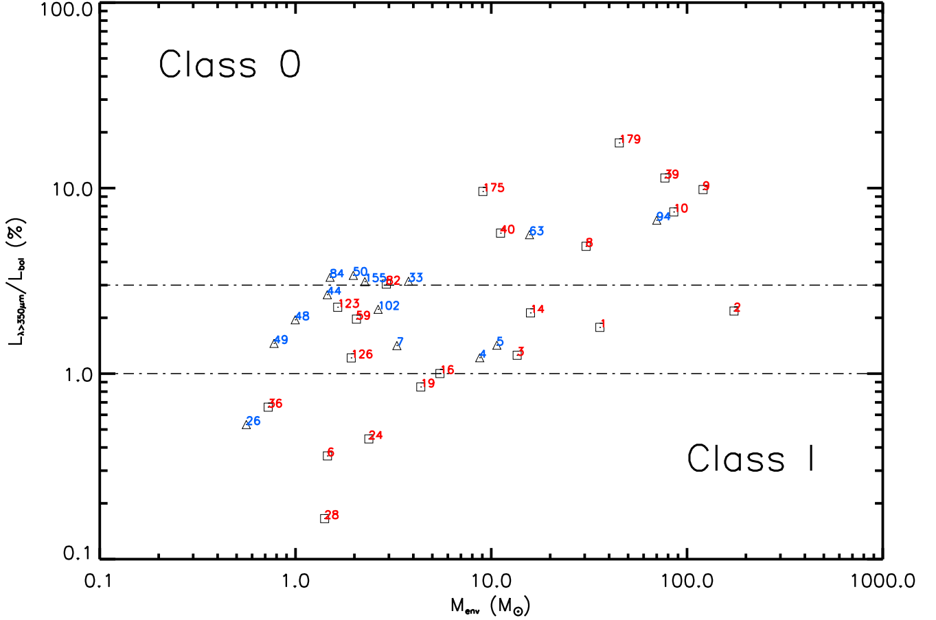
Fig. 15: L_{\lambda>350\mu m}/L_{bol} versus M_{env} . The dotted-dashed lines represents the L_{\lambda>350\mu m}/L_{bol} limits between Class 0 and Class I from Bontemps et al. (2010a) and sources are color-coded depending on their location: red squares for sources inside the PDR, blue triangles for outside
