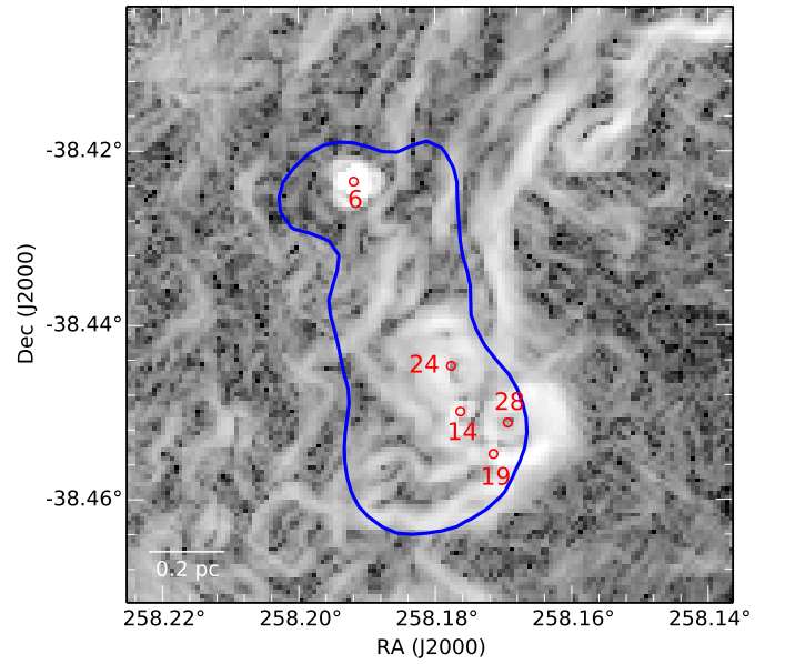
Fig. 22: Condensation 4: same as for Figure 19
