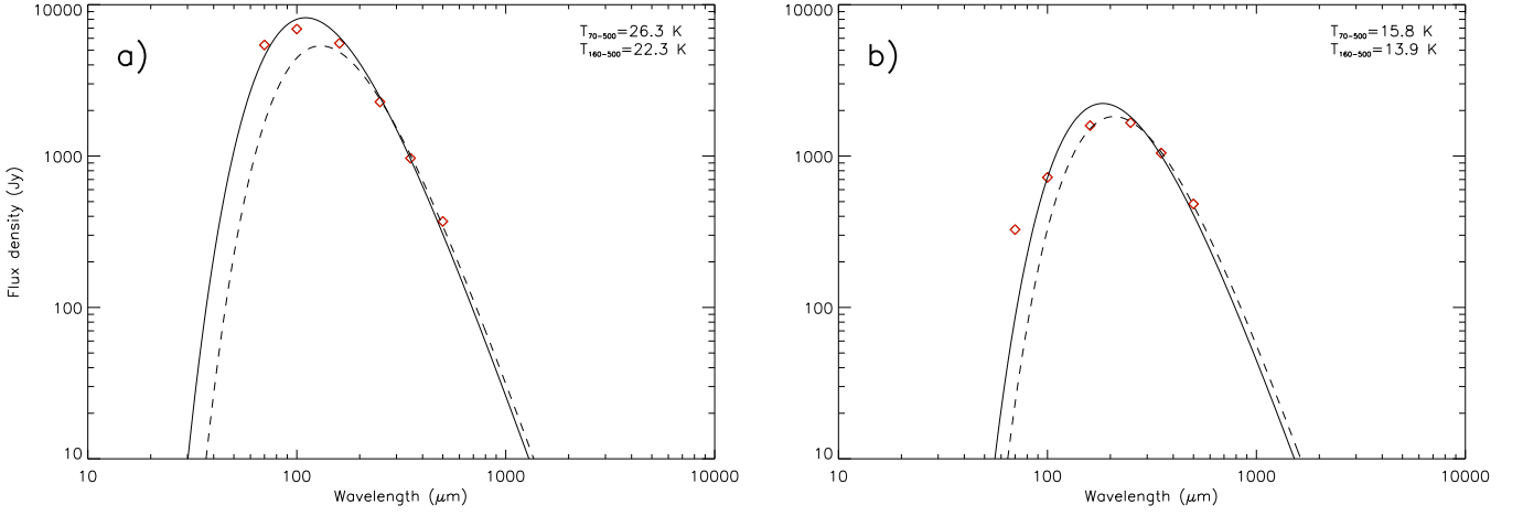
Fig. 2: (a) SED fitting for the pixels giving the highest temperature. The continuous curve represents the fit made with all Herschel fluxes and dashed curved is the fit obtained by the method of Hill et al. (2012). (b) Same for the pixel giving the lowest temperature. No background is subtracted in both cases
