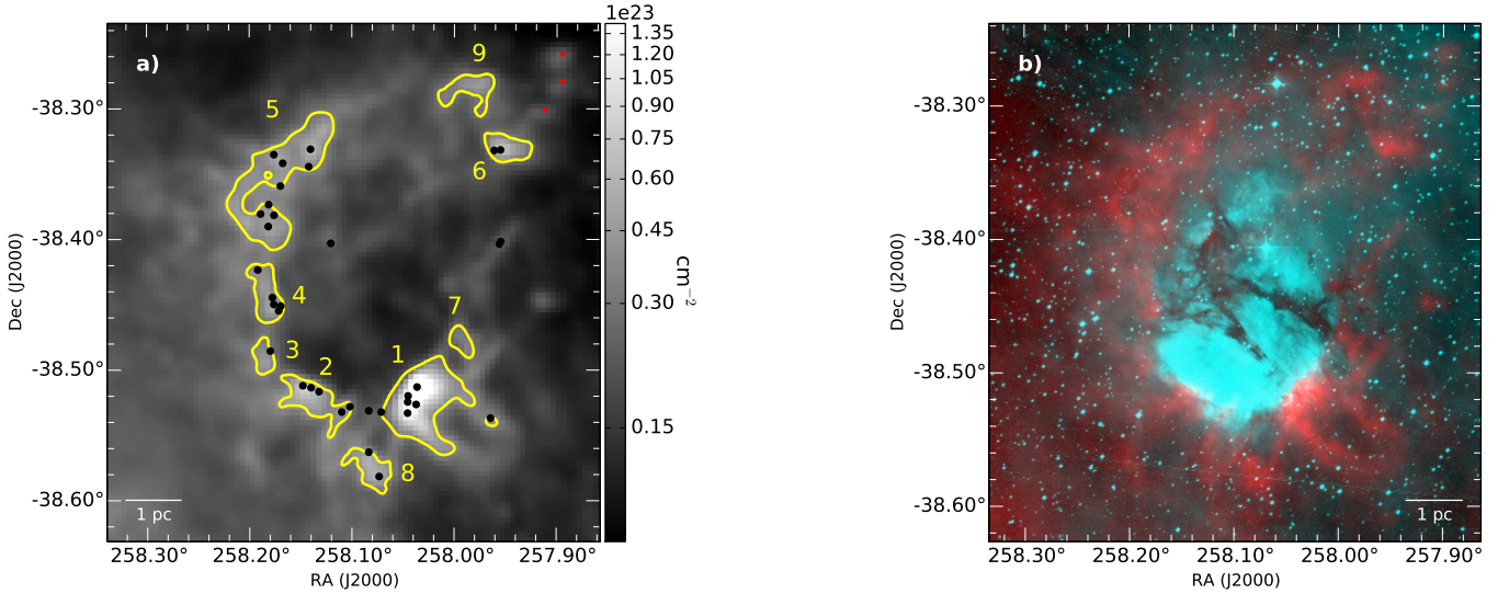
Fig. 5: (a) On logarithmic scale, H 2 column density map of RCW 120 at 36''6 resolution with 870 μm emission from LABOCA (in yellow contours), the final sample of sources (black dots) and the three prestellar clumps (red dots). Condensations observed at 870 μm are identified following the labelling in DEH09. The density values range from 7 \times 10^{21} \text{ cm}^{-2} to 4 \times 10^{23} \text{ cm}^{-2} . (b) High resolution H 2 column density map of RCW 120 at 18''2 resolution (in red) and H \alpha emission (in blue) from the SuperCOSMOS H \alpha Survey. The column density values range from 7 \times 10^{21} \text{ cm}^{-2} to 9.4 \times 10^{23} \text{ cm}^{-2} .
