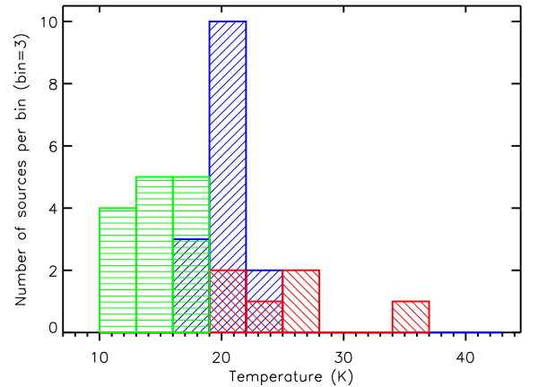
Fig. 14: Histogram of the temperature color-coded according to L_{\lambda \geq 350\mu\text{m}}/L_{\text{bol}} in green for Class 0, red for Class I and blue for uncertain cases
