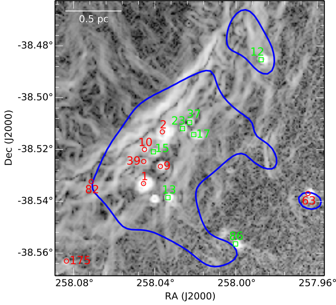
Fig. 19: Condensation 1 and 7: 870\mu\text{m} emission (countours) superimposed on the gradient image of the Herschel PACS 70\mu\text{m} emission. Sources are identified with their getsources identification number. Sources coded with a red circle are those discussed (among the sample of 35 sources). The green square sources are detected but not discussed due to a lack of Herschel measurements (see text)
