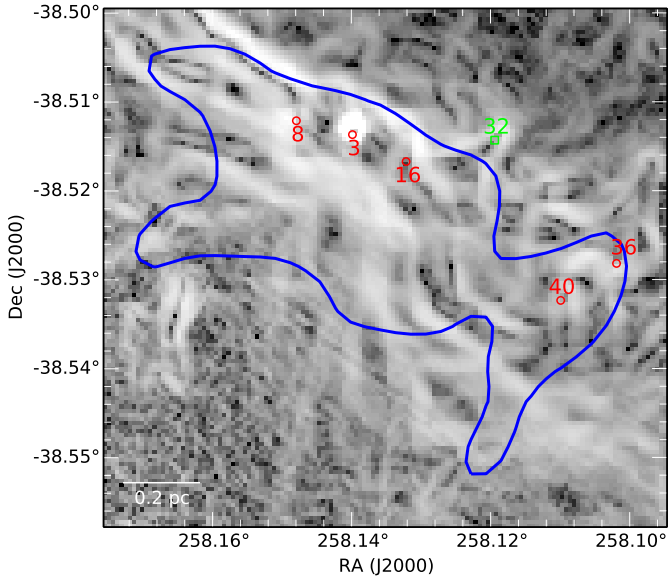
Fig. 20: Condensation 2: same as for Figure 19
