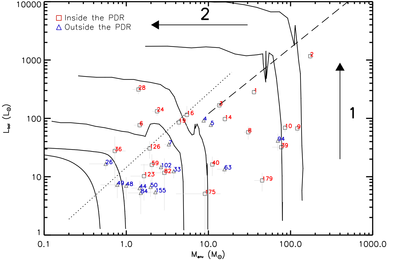
Fig. 16: L_{\text{bol}} versus M_{\text{env}} . Evolutionary tracks are adapted from Saraceno et al. (1996) and Molinari et al. (2008) . Labeled arrows indicate (1) the accretion phase and (2) envelope cleaning phase. Sources are coded as a function of their location with respect to the PDR : red squares sources are for the ones observed towards the PDR and blue triangles for those outside. Error bars for L_{\text{bol}} and M_{\text{env}} are shown by gray lines
