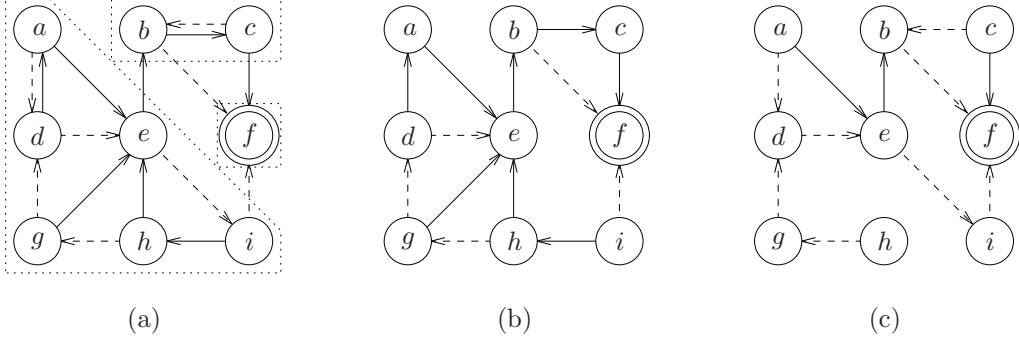
Figure 4: Sequence based on strongly connected components. (a) The graph has three strongly connected components C_1 = \{f\} , C_2 = \{b, c\} , C_3 = \{a, d, e, g, h, i\} . (b) The first step is S_1 = \{b, d, f, g, h, i\} , and only the nodes of S_1 can route according to \mathcal{R}_1 or \mathcal{R}_2 . (c) The second step is S_2 = \{a, c, e\} , and only the nodes of S_2 can route according to \mathcal{R}_1 or \mathcal{R}_2 .
