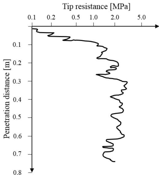
Figure 1. Example of penetration test (Benz-Navarrete (2009)).
