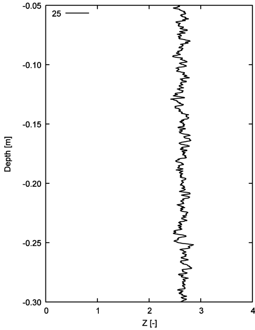
Figure 5. Coordination number versus penetration distance.
