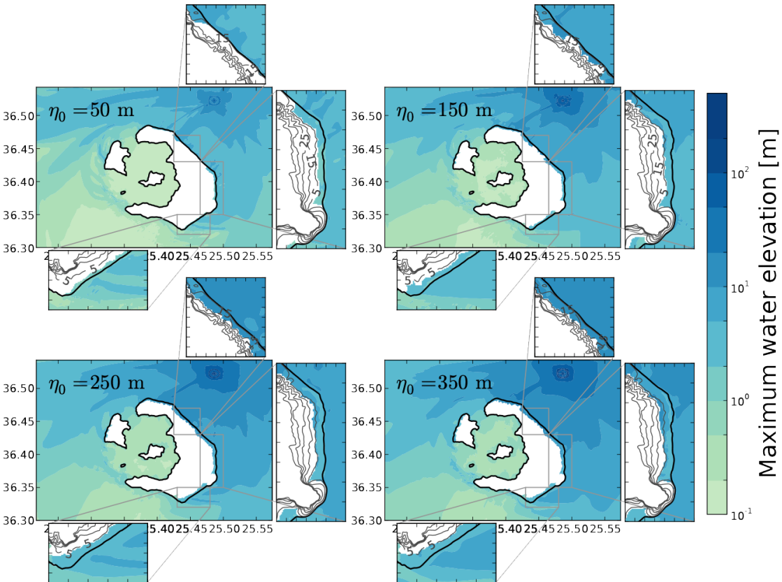
Fig. 9. Results of numerical calculations of the Kolumbo explosion generating tsunami. Maximum wave amplitudes around Santorini for several \eta_0 with zooming in the key coastal areas. Note, that the colour scale is logarithmic. Black thick solid line represents the original coastlines. Thin black lines in zooms are topography contours with 10 m interval starting at 5 m. Inundation of most east coast of Santorini is visible for all four scenarios.
