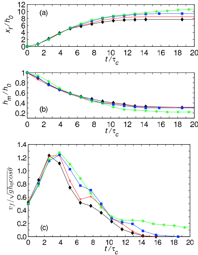
Figure 11. Normalized (a) location of the front x_f/h_0 , (b) maximum thickness of the flow (i.e., thickness at the upper wall) h_m/h_0 , and (c) velocity of the front v_f(t)/c_0 ( 22^\circ ) ( c_0 = \sqrt{gh_0 \cos \theta} = 1.128 \text{ m.s}^{-1} ), with h_0 = 0.14 \text{ m} , as a function of time t/\tau_c , where \tau_c = \sqrt{h_0/(g \cos \theta)} , = 0.124 \text{ s} for inclination angle \theta = 22^\circ over a rigid bed h_i = 0 (diamond), and erodible bed of thickness h_i = 1.82 \text{ mm} (cross), h_i = 3.38 \text{ mm} (square), and h_i = 4.6 \text{ mm} (star).
